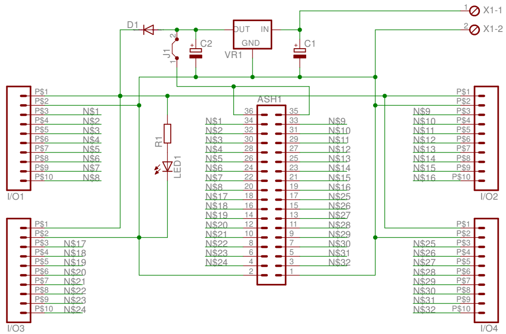
32 bits I/O shield for DCCPP central commander with Arduino Mega.
